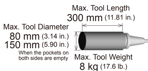
H.Plus-300 PC15 320T magazine Option
